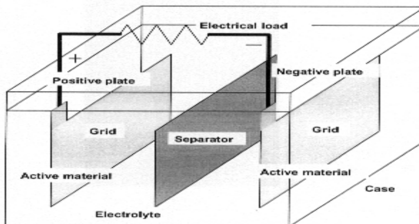
Figure 1. Battery cell composition
